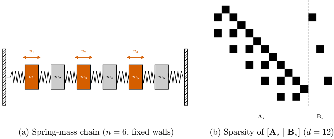
Figure 12: The coupled spring-mass chain benchmark. (a) n masses on linear springs between fixed walls; every other mass is actuated (highlighted, with control force u_j ). (b) The induced sparsity pattern of \Theta_* = [\mathbf{A}_* | \mathbf{B}_*] for n = 6 ( d = 12 ). The drift block \mathbf{A}_* is banded – position rows carry a single unit entry and velocity rows couple only to a mass and its neighbours (three drift nonzeros); with one control entry per actuated mass in \mathbf{B}_* , the largest joint row support is a fixed s = 4 regardless of d .
