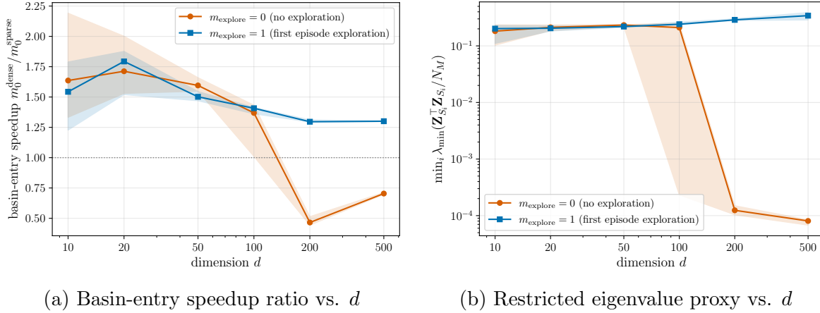
Figure 7: Greedy certainty equivalence ( m_{\text{explore}} = 0 ) versus one initial exploration episode ( m_{\text{explore}} = 1 ), across dimension (medians across 20 seeds, IQR shaded). (a) The basin-entry speedup dives below 1 without initial exploration at d \geq 200 , i.e., the sparse advantage reverses. (b) The control-block restricted-Gram minimum eigenvalue collapses without and stays away from zero with the initial exploration.
