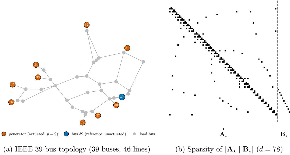
Figure 14: The IEEE 39-bus power grid. (a) The New England topology with 39 buses, 46 lines, the nine actuated generators (highlighted) and bus 39 as the unactuated reference. (b) The induced sparsity of \Theta_* = [\mathbf{A}_* \mid \mathbf{B}_*] ( d = 78 , 3.2% nonzero). As for the chain the angle rows carry a single entry, but the frequency rows now scatter over the irregular grid graph rather than forming a band. \mathbf{B}_* has one entry per actuated generator.
