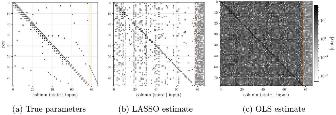
Figure 16: Topology recovery on the IEEE 39-bus grid after the initial episode: log-magnitude heatmaps of \Theta = [\mathbf{A} \mid \mathbf{B}] for a median-regret seed. (a) The true parameters, whose support encodes the grid’s wiring (3.2% dense). (b) Our sparse (LASSO) estimate after the single exploration episode ( H = 50 samples): 82% of entries are exactly zero and the coupling skeleton is already recognisable. (c) The dense (least-squares) estimate from the same data: underdetermined, it returns noise at the magnitude of the largest true couplings. The vertical line separates the state block from the input block. The control block is noisy for both estimators, showing the drift-control asymmetry of Figure 15b. By m = 1000 both estimators recover the support almost perfectly.
