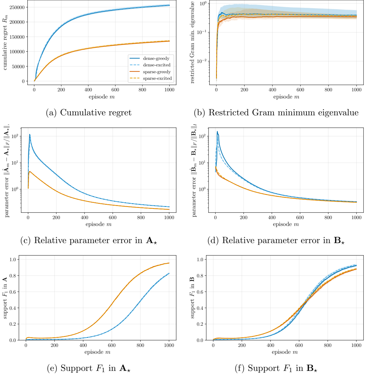
Figure 6: Per-episode diagnostics at the largest synthetic dimension ( d = 500, p = 250 ). All show the median and the IQR shaded, and the legend in panel (a) applies to all. (a) Cumulative regret separates the sparse from the dense agents early, with non-overlapping bands. (b) The minimum eigenvalue of the (restricted) empirical Gram matrix is comfortably bounded away from zero after the exploration episode, suggesting identifiability throughout. (c)(d) Relative parameter error of the drift and control blocks: the sparse estimator peaks lower and descends earlier in both, but its final advantage concentrates in the drift block. (e)(f) LASSO recovers the drift support almost exactly, while false positive entries in the control block cap both methods.
